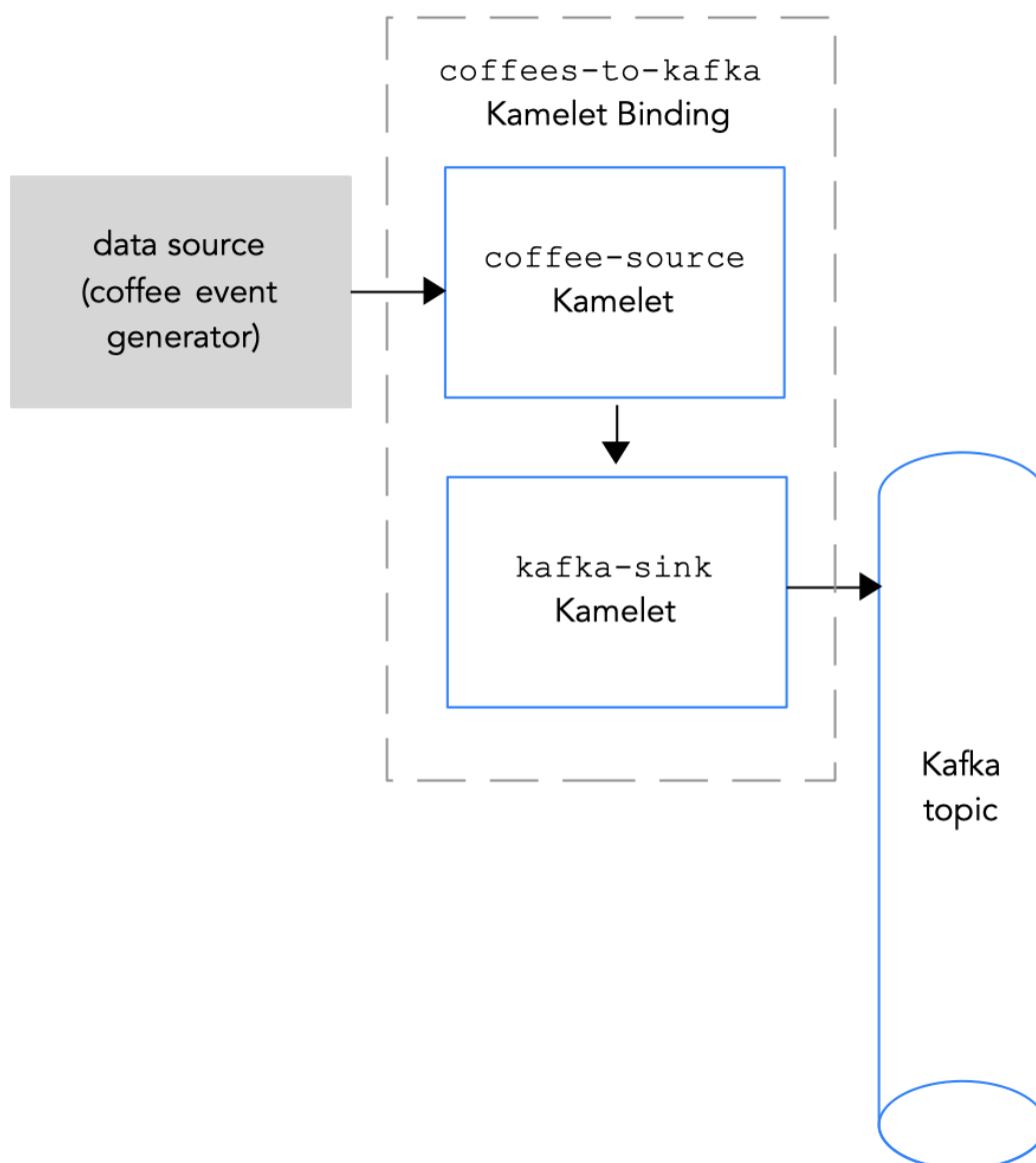
Figure 2.2 Connecting a data source to a Kafka topic
