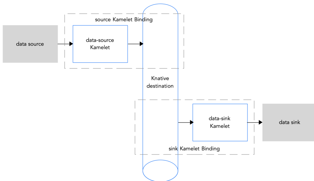
Figure 3.1: Data flow with Kamelets and a Knative channel
