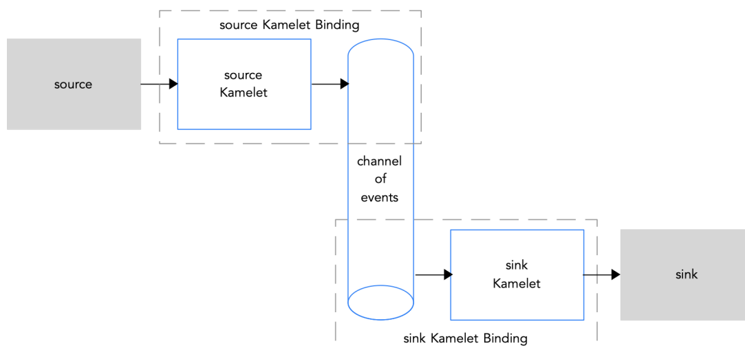
Figure 1.3: Connecting source and sink Kamelets to a channel of events
