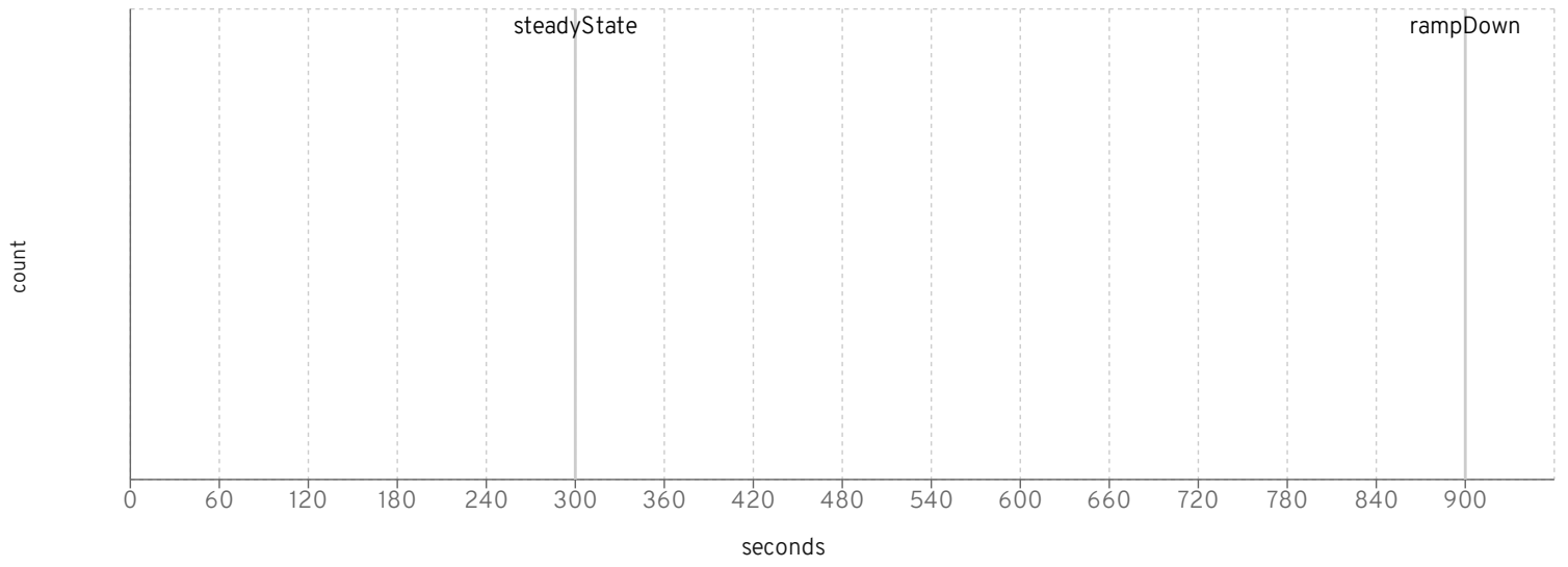
supplierWorker queue
