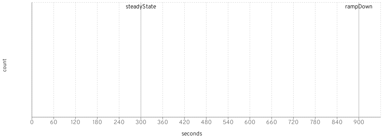
supplierWorker threads
