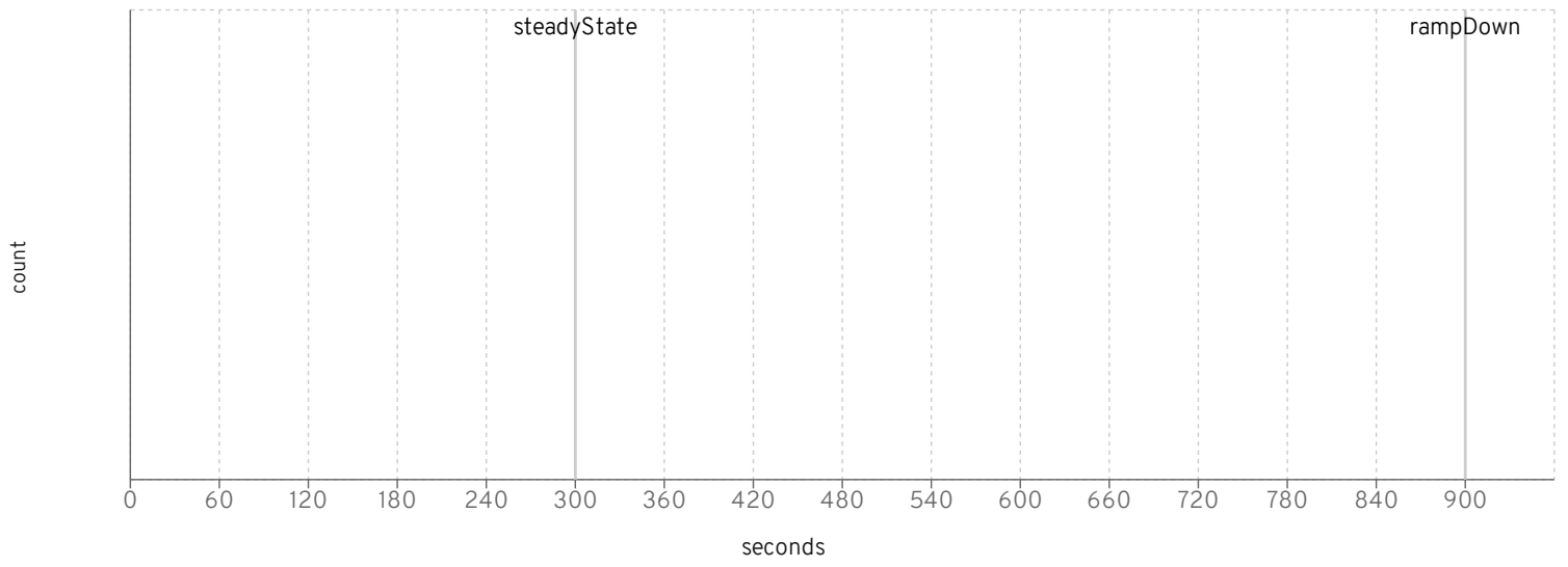
supplierWorker queue
